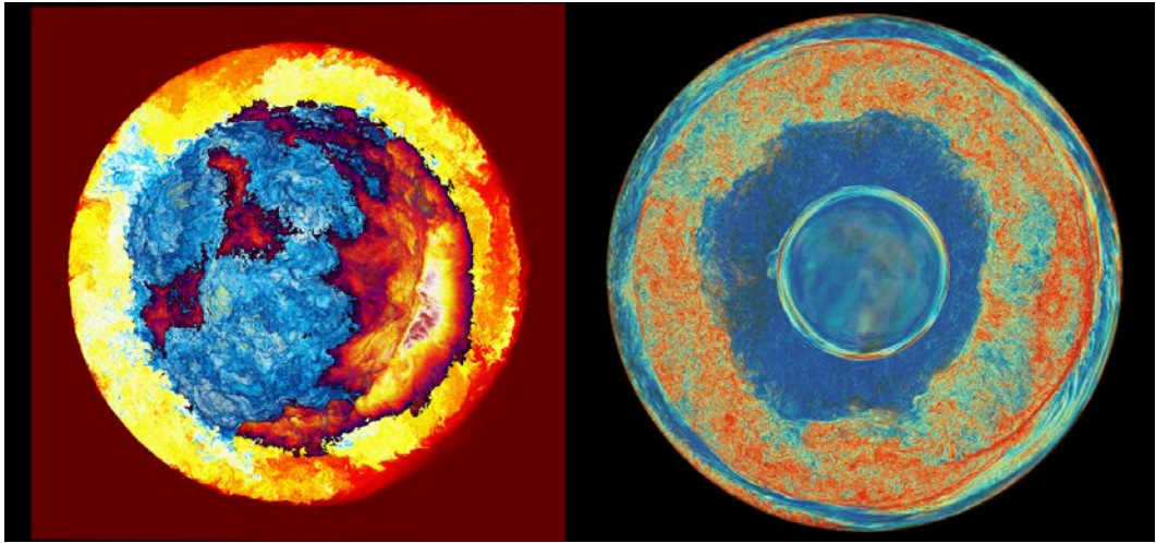
Figure 1d. The same two volume-rendered views of the far hemisphere of the simulated interior of a 2 M_{\odot} AGB star of the early universe, with metallicity Z = 10^{-5} , but now the renderings are at time 2699 min. A violent wave of combustion of entrained, H-rich gas is now seen at the lower right, about to cross the star, pulling down large concentrations of H-rich fuel. At this stage, the presence of our outer bounding sphere becomes strongly felt, and our simulation can no longer be trusted. All the hydrogen within the bounding sphere is quickly consumed after the combustion wave reaches the opposite side of the star. We are now testing a new code that will be able to move the bounding sphere outward a factor of 2 in radius.
