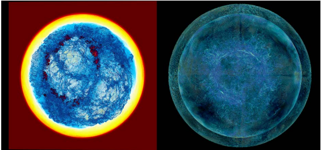
Figure 1c. The GOSH (see text) has created a hydrogen enriched layer floating at the top of the convection zone driven by helium burning in the turbulent gas near the carbon-oxygen core.
