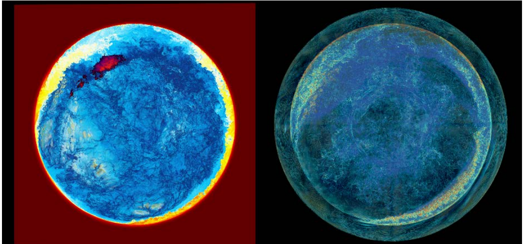
Figure 1b. A global, tsunami-like wave driven by burning ingested hydrogen traverses the star.
