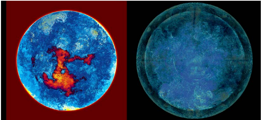
Fig. 1a. Two volume-rendered views of the far hemisphere of the simulated interior of a 2 M_{\odot} AGB star of the early universe, with metallicity Z = 10^{-5} . At the left, we see the concentration of H-rich gas entrained into the convection zone above the helium burning shell during the H-ingestion flash. The material of the convection zone and of the degenerate carbon-oxygen core is transparent. Where the clipping plane passing through the center of the star meets the top of the convection zone, a clearly visible circle in both images, we see the entrained gas in cross section. Outside the circle, the concentration is unity, and it appears red. As the concentrations decrease, colors go from red to yellow, white, aqua, and finally dark blue. We see the dome of the spherical convection zone boundary in projection, and where descending entrained H is burning, we represent the released energy by colors that indicate a flame, with the energy increasing as the colors go from purple to red and finally to yellow and white. In the image at the right, we see the magnitude of vorticity. Vorticity is confined mainly to the inside of the convection zone, from about radius 11 Mm to 28 Mm. The bottom of this convection zone, which is clearly visible as a circular feature, is very near the surface of the C-O core. Between the top of the convection zone and the outer bounding, reflecting sphere, there is very little gas motion, even though shear right at the bounding sphere makes it visible in this very sensitive variable. A burst of strong vorticity and high turbulence is visible near the bottom of the image, where a rising gust driven by recent burning of ingested H is pushing against the top of the convection zone and driving wedges of entrained gas visible in yellow at the bottom of the left image. This is the beginning of a GOSH (see text).
