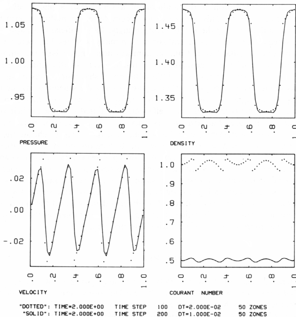
FIG. 4. Results after two sound crossing times for a nonlinear standing wave in a box with reflecting walls. The solid lines represent results obtained from the explicit version of the scheme at a Courant number of 0.5 while the dotted line was obtained using the implicit-explicit hybrid method at a Courant number of 1 based on the ambient sound speed. Note from the plot of the Courant number that half of the wave is being calculated implicitly and half explicitly without producing any noise in the solution. Since both the implicit and explicit schemes are exact at a Courant number of 1, the results obtained with the hybrid method are somewhat more accurate than those produced by the purely explicit method.
