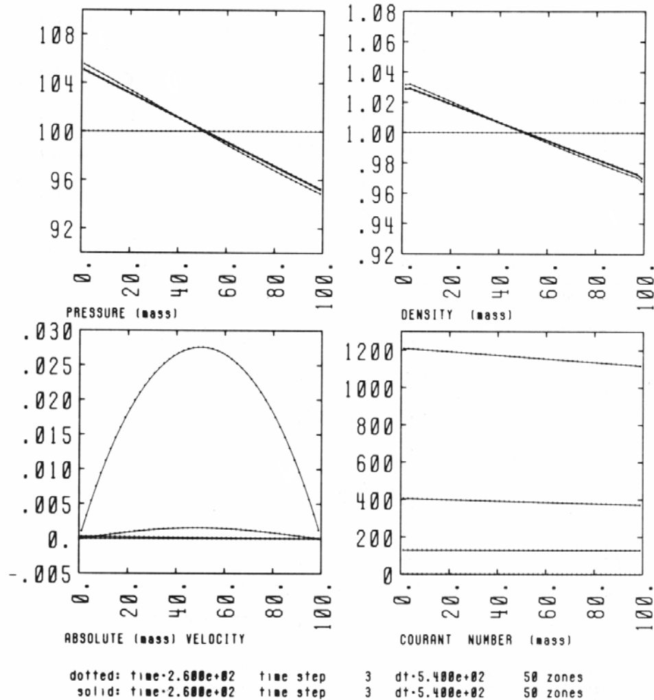
FIG. 12. The relaxation to a steady state of a uniform density gas with a constant gravitational acceleration to the left. Results after each of the first three time-steps as well as the initial distribution are plotted. The final two curves are indistinguishable, showing that the steady state has been obtained after only two time-steps.
