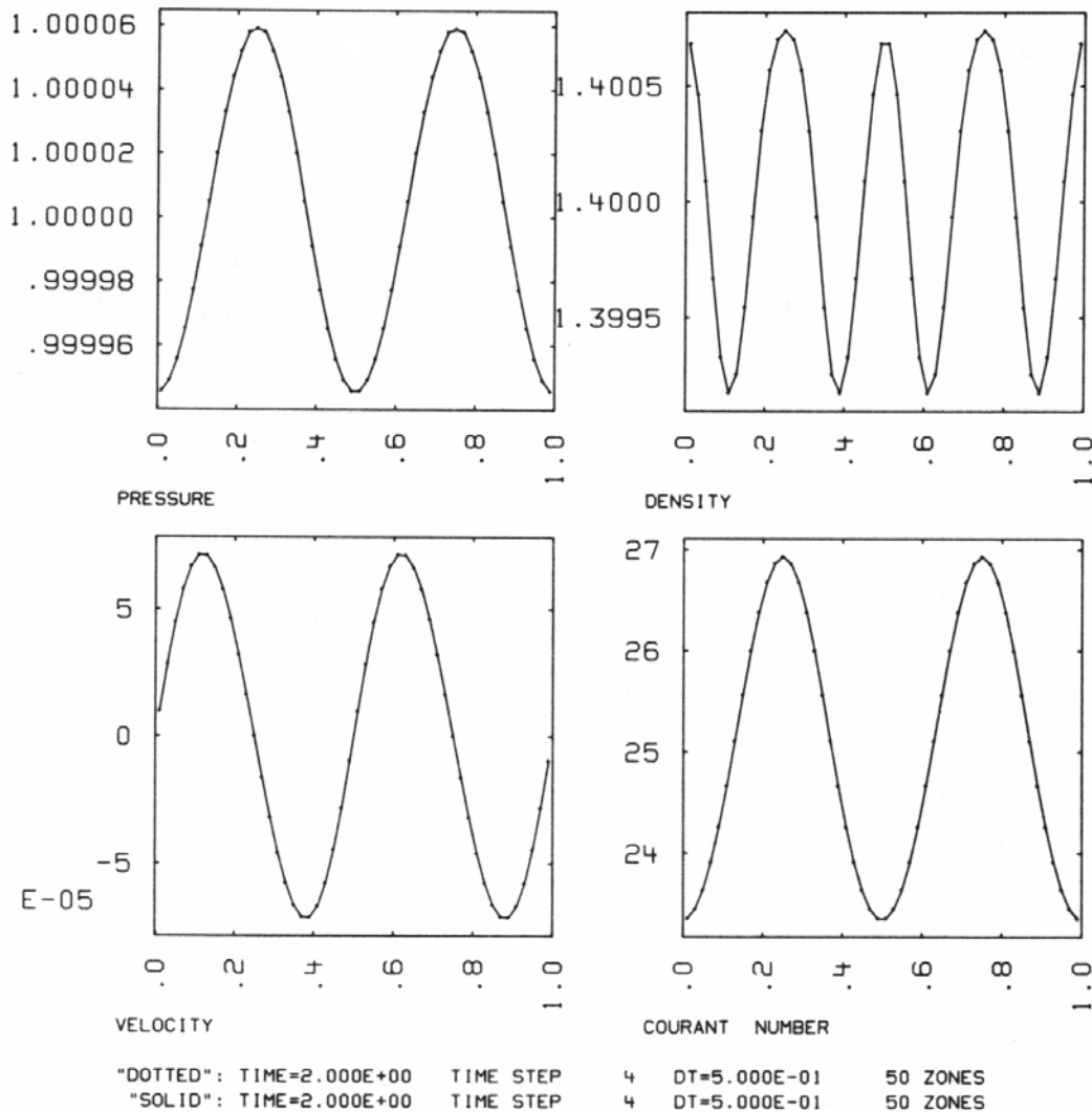
FIG. 7. Results for a nonlinear standing wave in a box obtained at a Courant number of 25. The wave is now moving 1 wavelength/time-step. As expected, the wave is strongly damped. The pressure and velocity are damped before the density, leaving an oscillation in the density of half the original wavelength where the wave deposited its energy while being dissipated.
