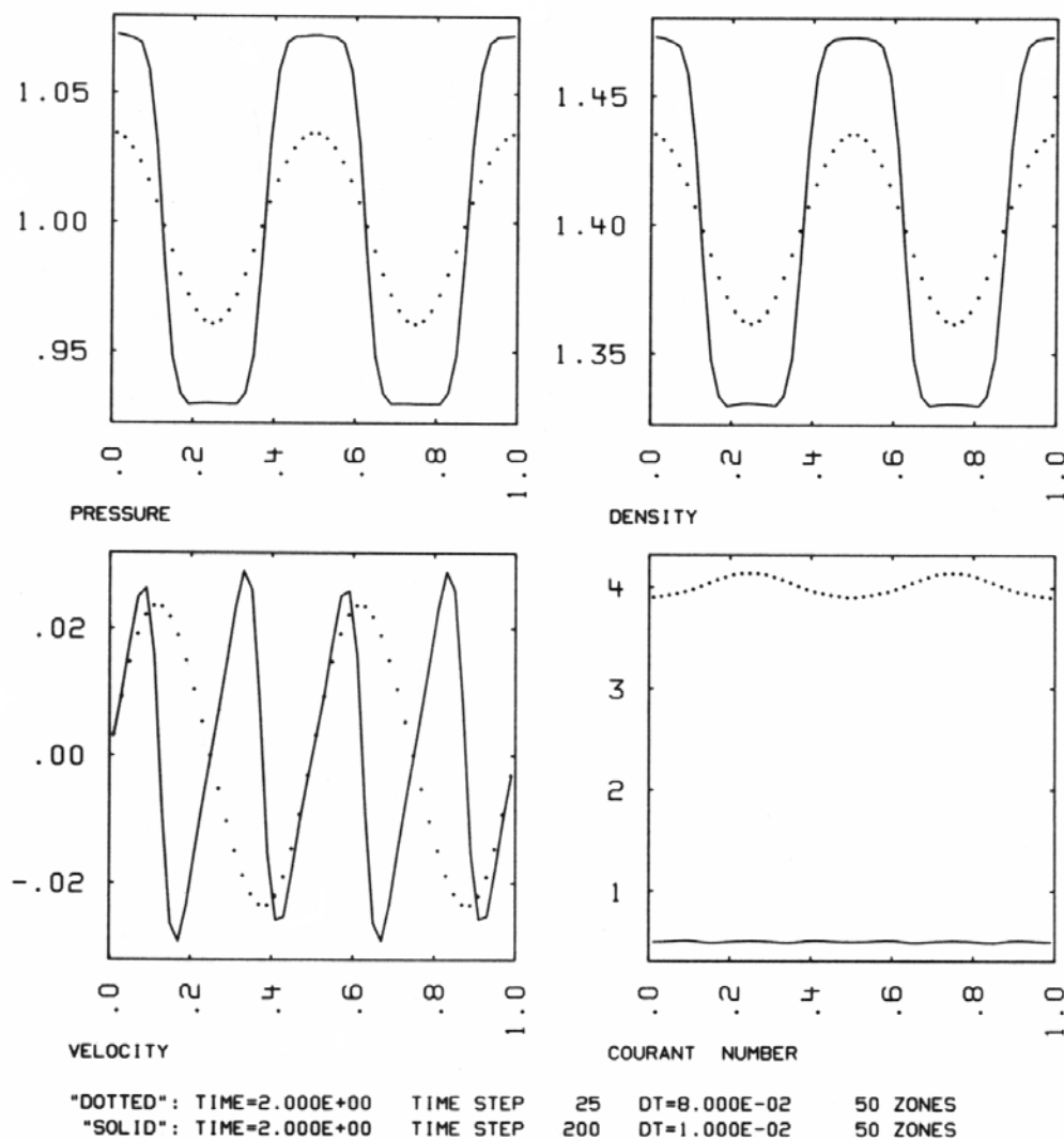
FIG. 6. Results for a nonlinear standing wave in a box obtained at a Courant number of 4. Now only the fundamental frequency remains and its amplitude has been damped noticeably.
