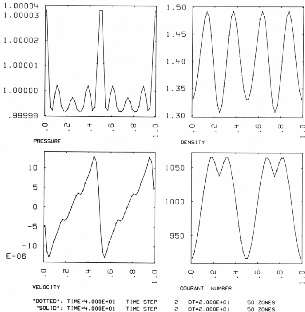
FIG. 8. Results for a nonlinear standing wave in a box obtained at a Courant number of 1000. For all practical purposes, the wave has been eliminated after two cycles except for the residual oscillation in the density. The wave is moving 40 wavelengths/time-step.
